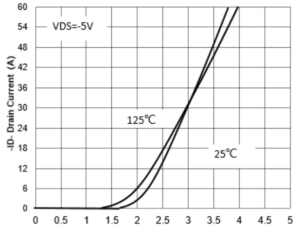
Figure8: -Vgs Gate-Source Voltage (V)
