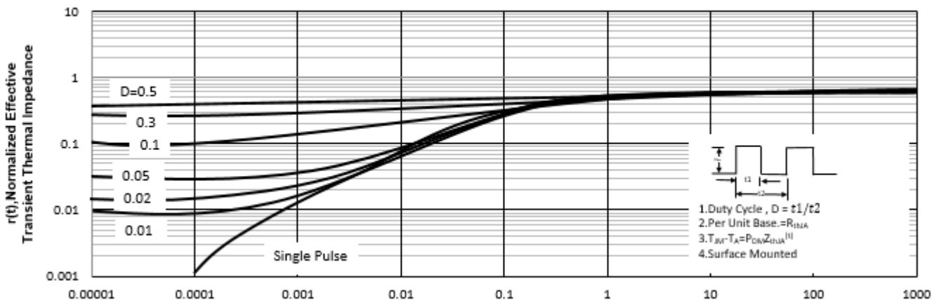
Figure10: Square Wave Pulse Duration (sec)
