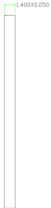
SIDE VIEW
